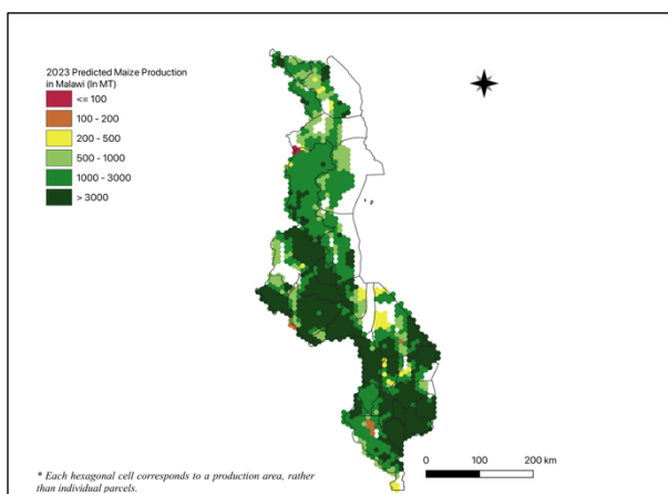
Figure 2. Malawi 2023 Maize production forecast.
