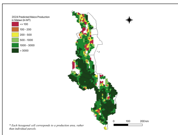
Figure 1. Malawi 2024 Maize production forecast.
